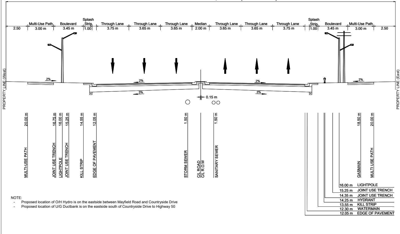
Arterial A2 - Recommended Cross-Section, Mid-Block (45 m ROW min)
