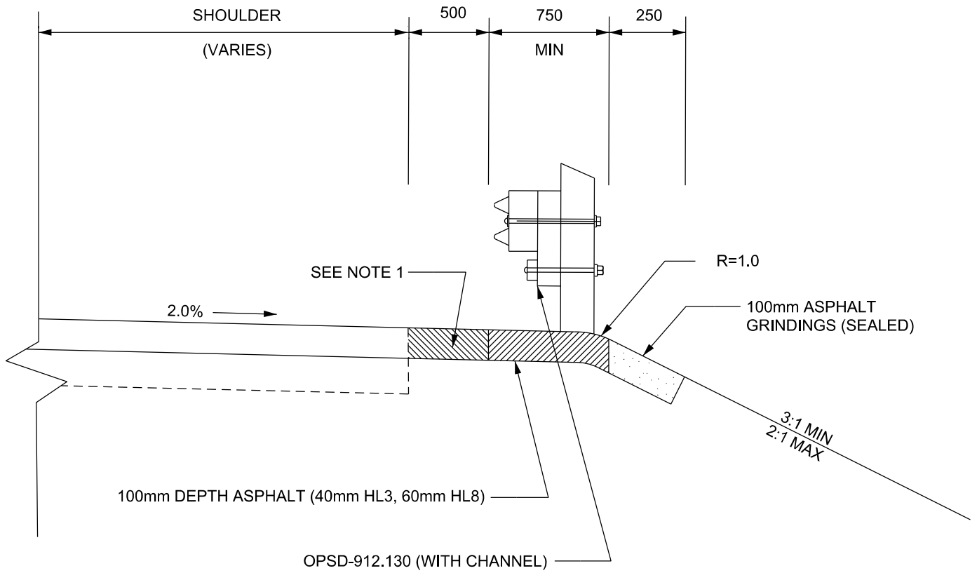
TYPICAL GUIDERAIL ARRANGEMENT
