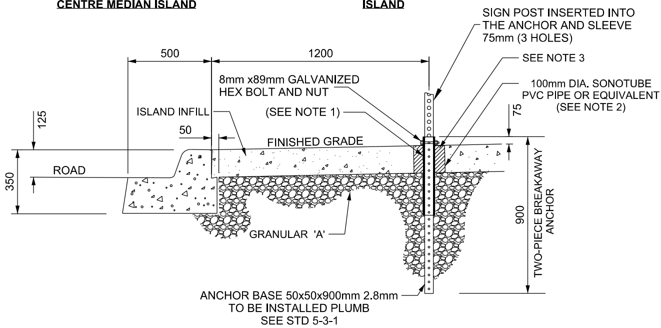
SECTION B-B
