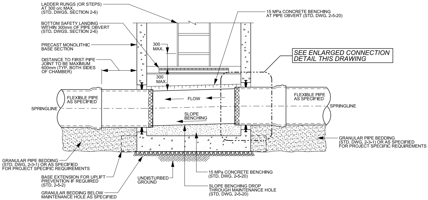
TYPICAL SMALL DIAMETER FLEXIBLE SEWER PIPE CONNECTION
