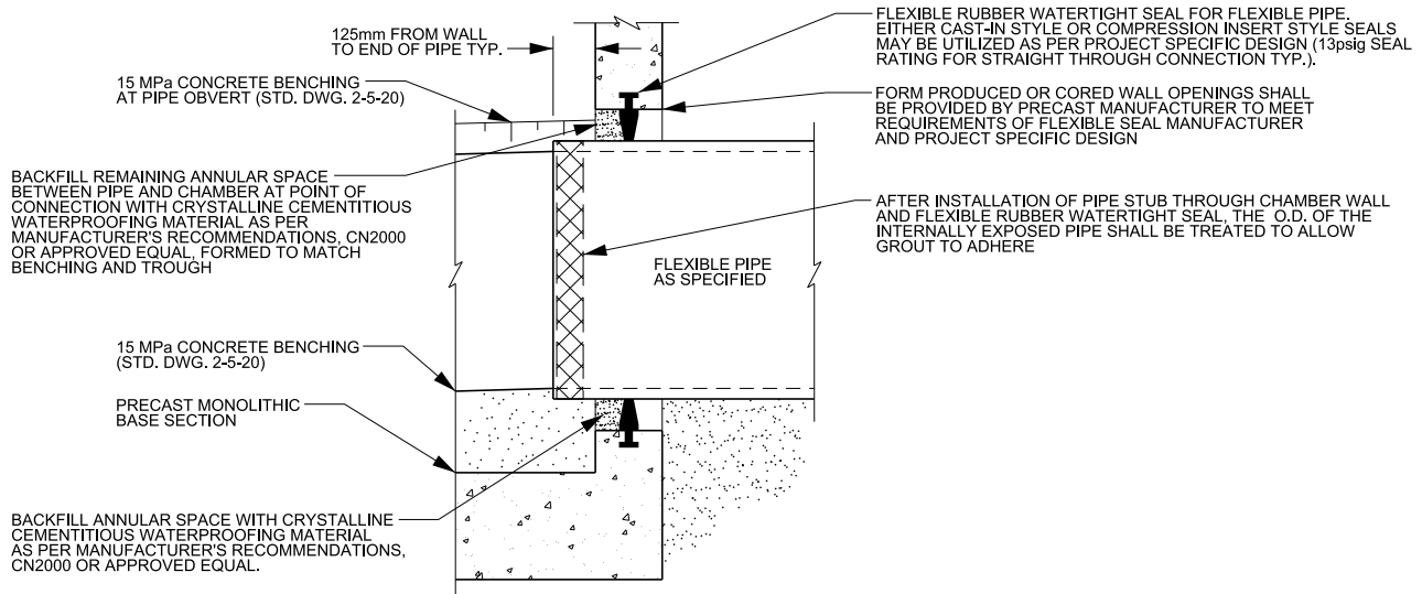
ENLARGED CONNECTION DETAIL
